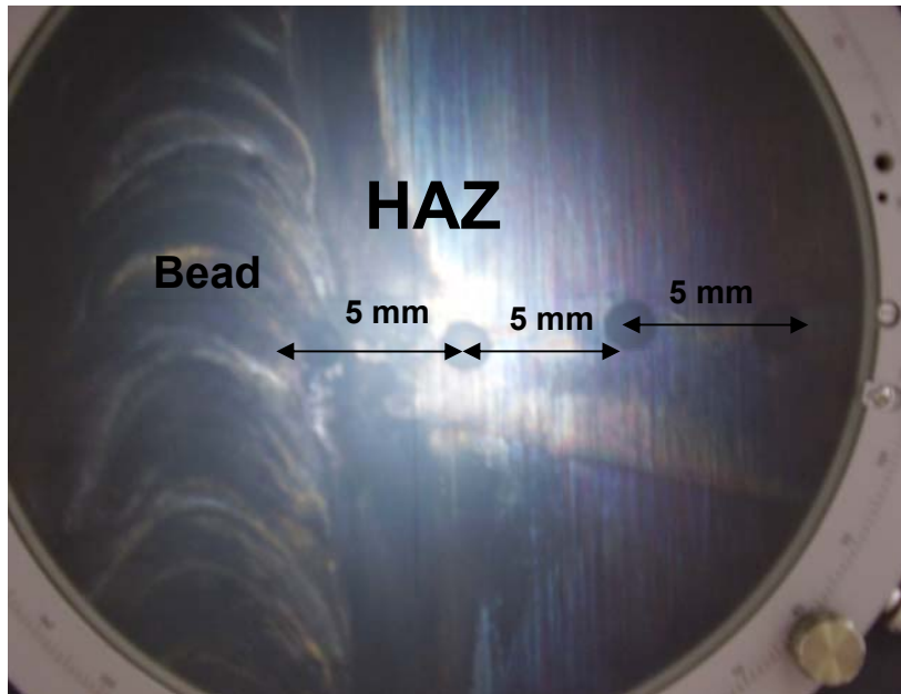
Figure 3: Distance thermocouples-bead.
